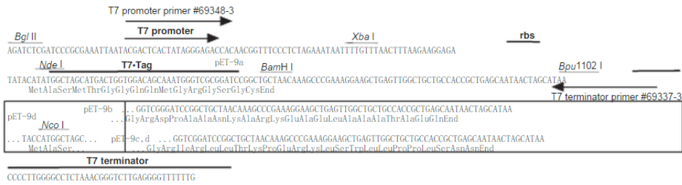
pET-9a-d cloning/expression region
